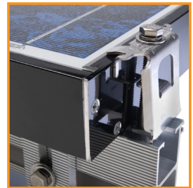
Grounding End Clamp
