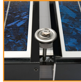
Grounding Mid Clamp
