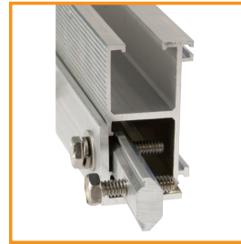
Grounding Splice Bar
